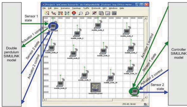
Figure 13 Interactive SIMULINK-OPNET co-simulation (see online version for colours)
