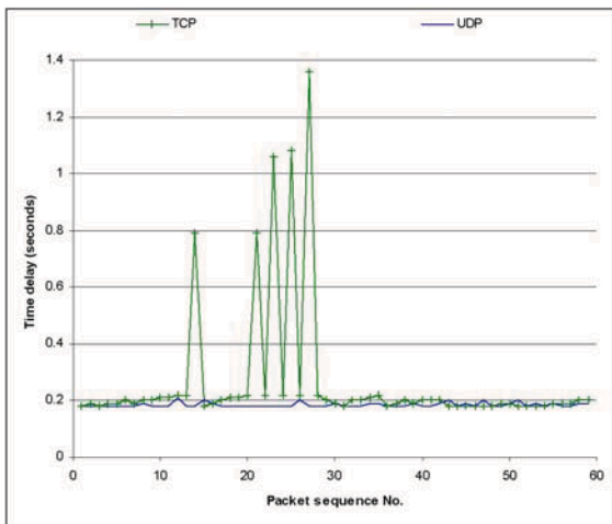
Figure 15 Comparison of delay and jitter between TCP and UDP (see online version for colours)
