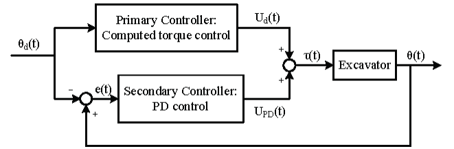
Figure 11 Control architecture
