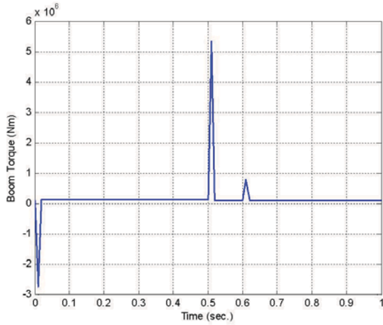
Figure 8 The boom torque (see online version for colours)
