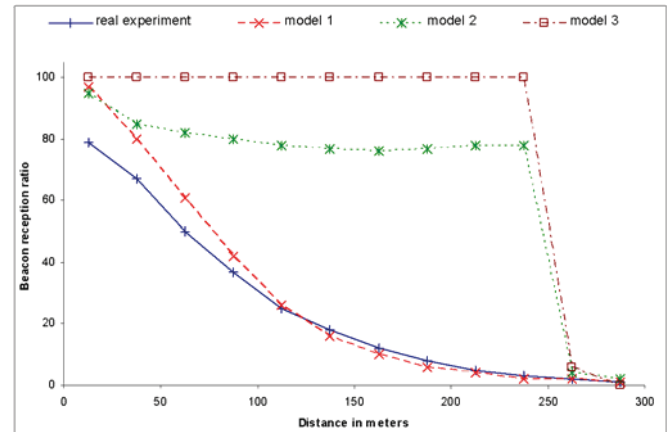
Figure 14 Comparison of three simulation models with real world experiment (see online version for colours)
