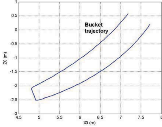
Figure 7 The bucket trajectory (see online version for colours)
