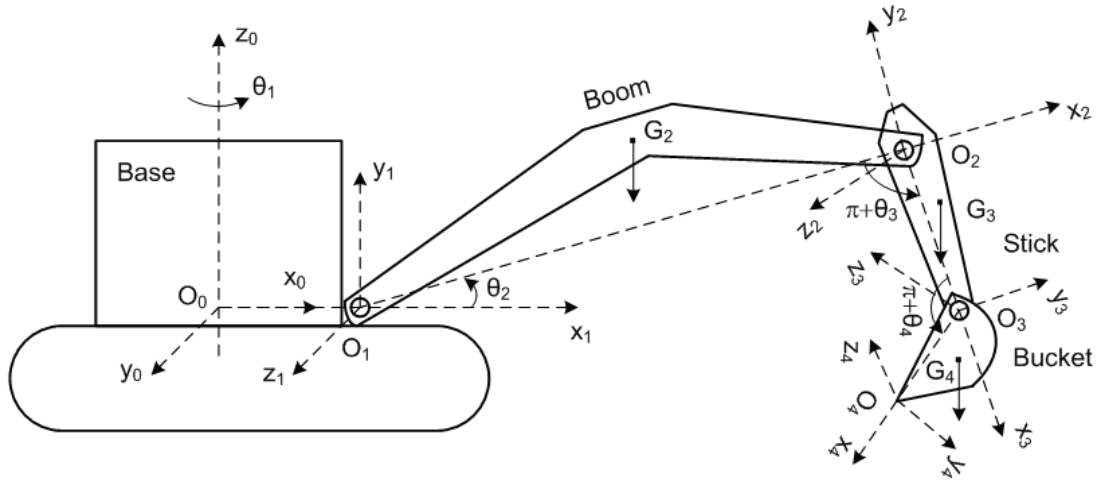
Figure 5 Schematic diagram of the excavator
