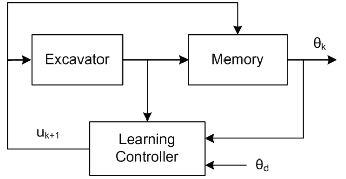
Figure 12 The iterative learning control scheme for the excavator
