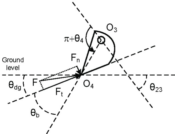
Figure 6 The interaction between the excavator bucket and the environment
