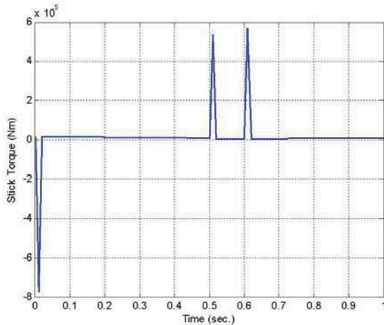
Figure 9 The stick torque (see online version for colours)
